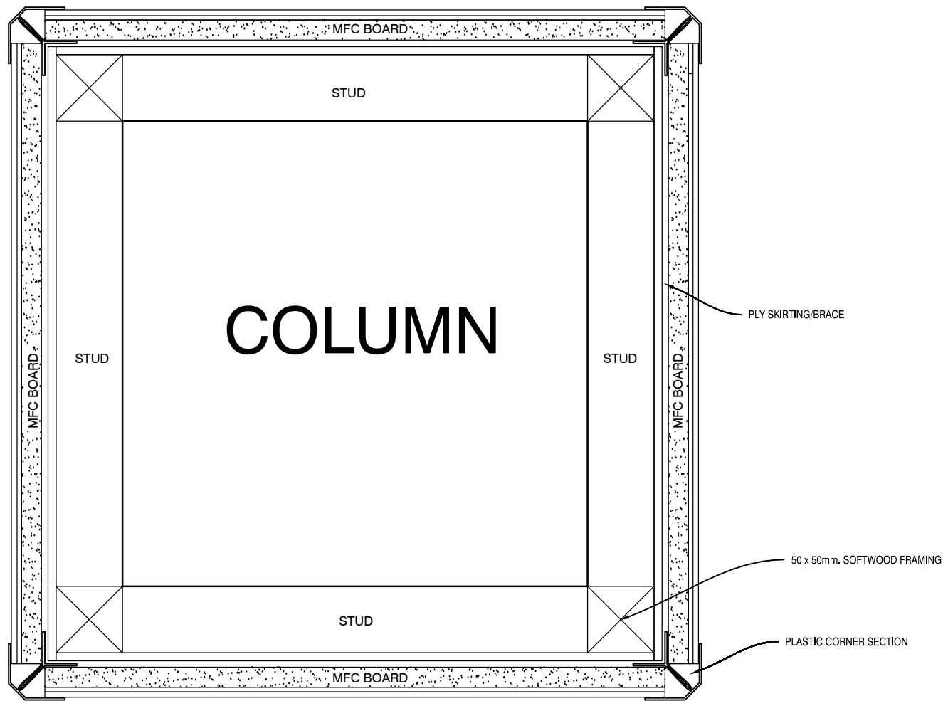
TYPICAL COLUMN DETAIL - PLAN
