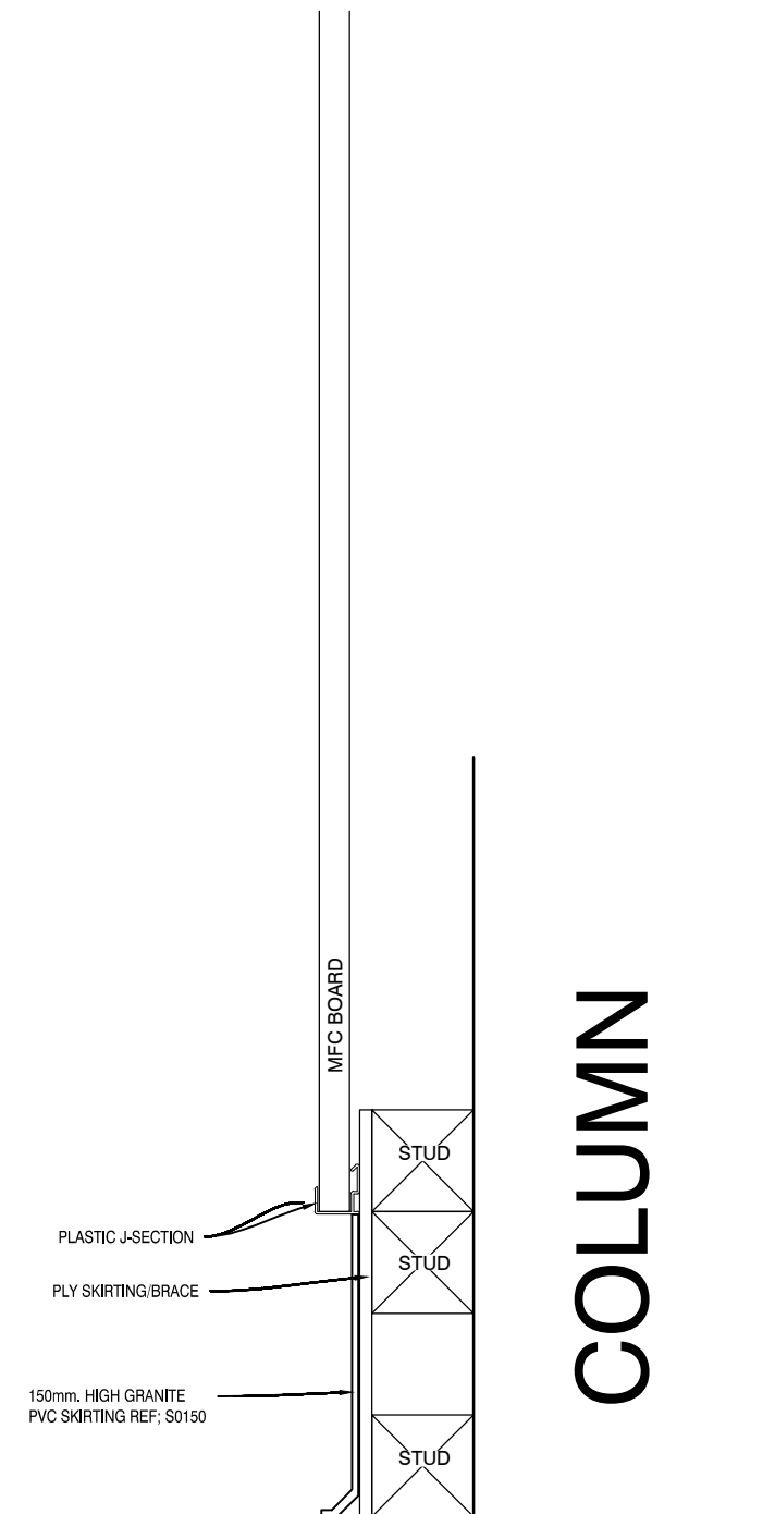
TYPICAL COLUMN DETAIL - SECTION
