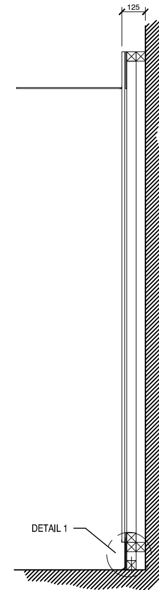
TYPICAL WALL CLADDING G.A.(1:20)
